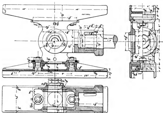
Figs. 1105-1107. Alligator Crosshead.
